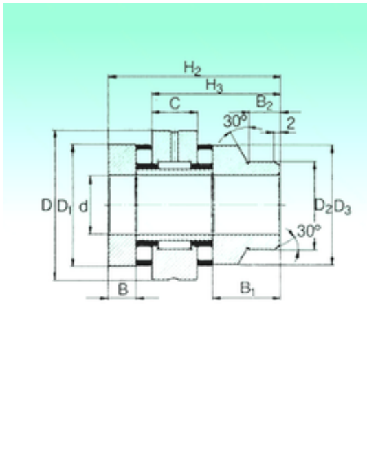
ZARN 50110 L TN Bearing 2D drawings and 3D CAD models
